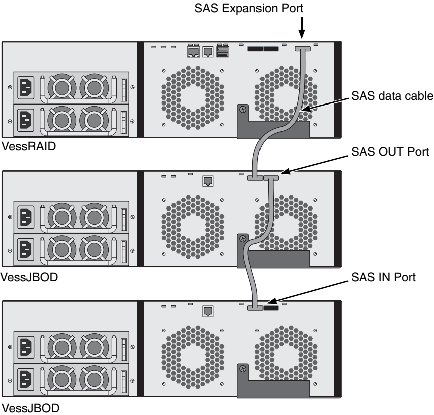
Figure 23. SAS JBOD expansion data connections
