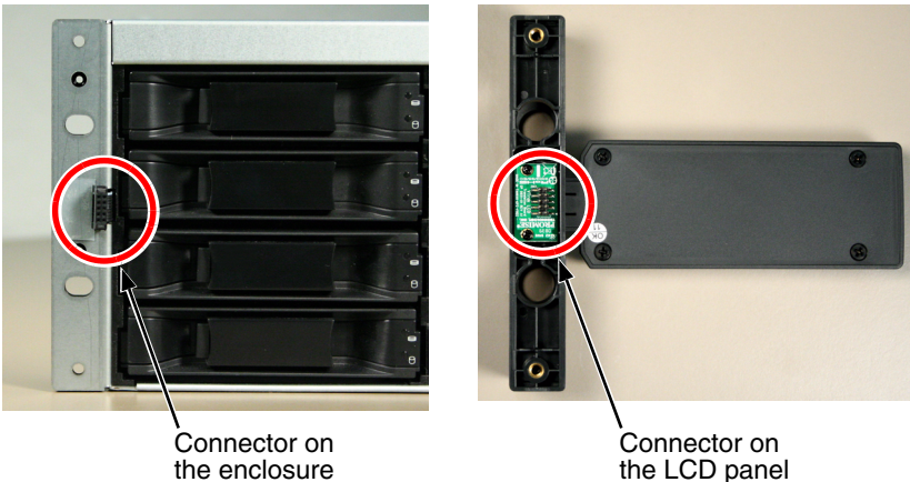
Figure 7. Align the connectors on the enclosure and the LCD panel
