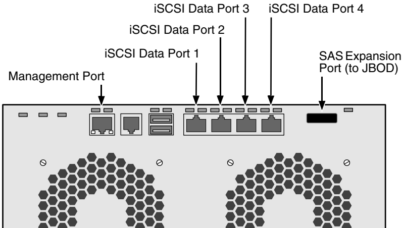
Figure 19. iSCSI DAS data and management connections
