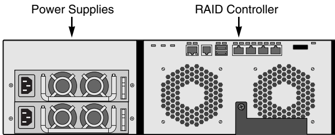
Figure 4. VessRAID 1840s rear view
