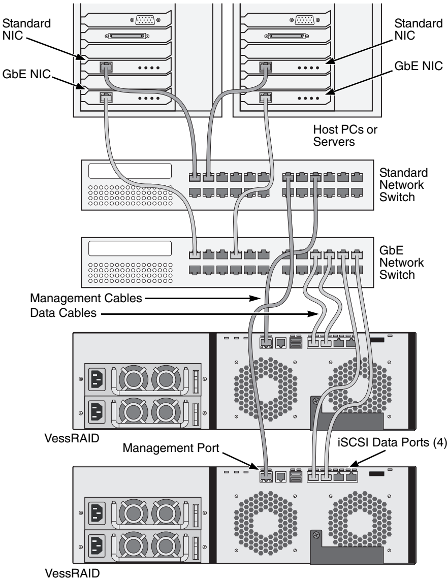
Figure 20. iSCSI SAN data and management connections
