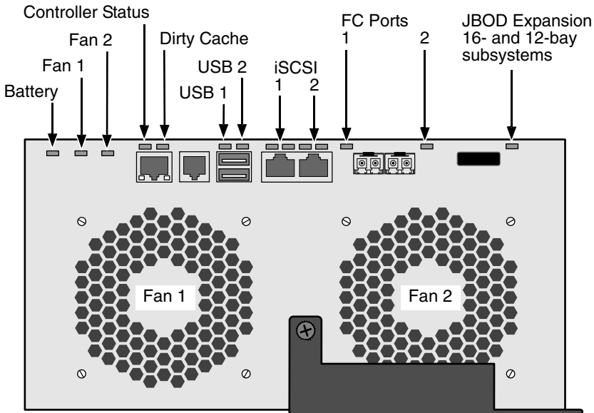
Figure 26. VessRAID FC Controller LEDs
