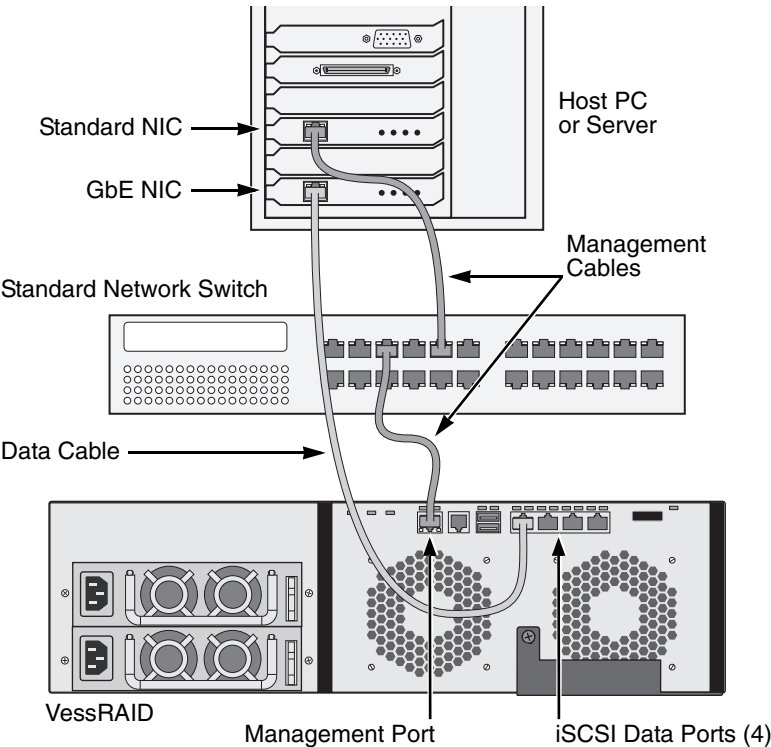
Figure 19. iSCSI DAS data and management connections
