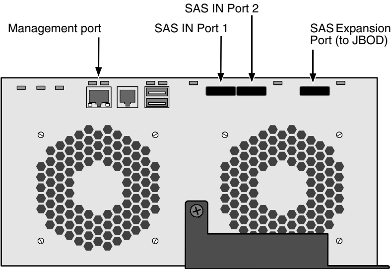
Figure 22. SAS DAS data and management connections
