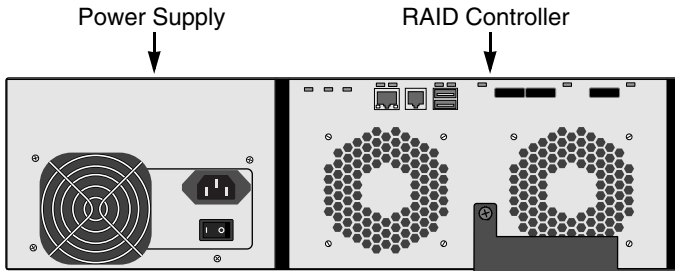
Figure 6. VessRAID 1740s rear view
