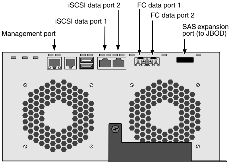
Figure 15. VessRAID FC data and management ports
