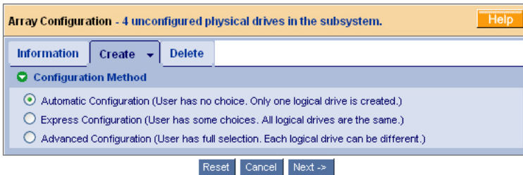
Figure 36. The Array Configuration menu
