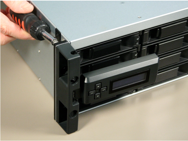
Figure 8. Attaching the LCD panel to the VessRAID enclosure
