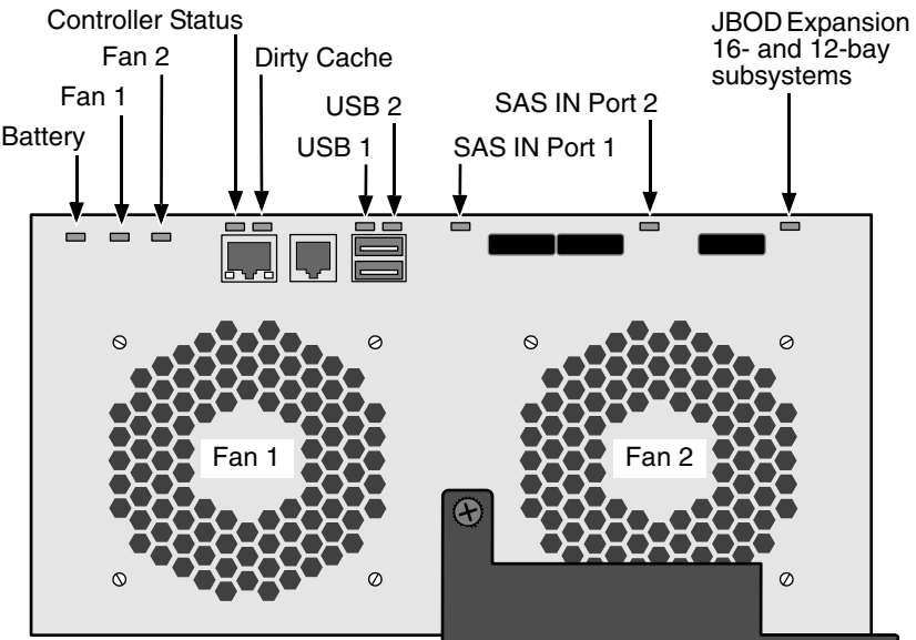
Figure 28. VessRAID SAS Controller LEDs
