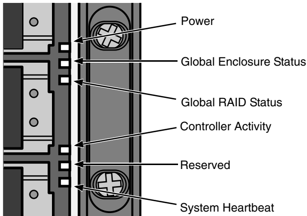
Figure 25. VessRAID front panel LED display
